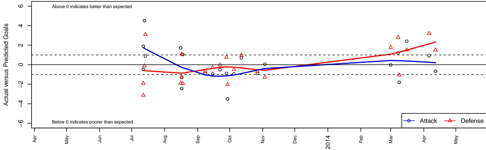
TFA Barcelona OR B02 Dots are actual minus expected GF (blue circles) and GA (red triangles). Blue line is smoothed change in attack strength. Red is smoothed change in defense strength.
